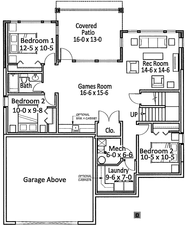
Lower Floor Plan 1436 Sq.Ft
