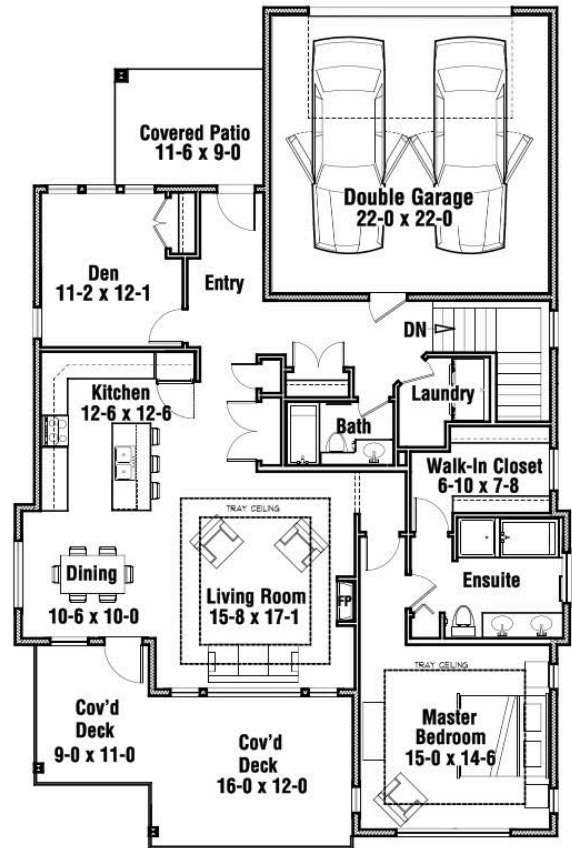
Main Floor Plan - 1615 Sq.Ft. 529 Sq.Ft Garage 266 Sq.Ft Cov'd Deck 162 Sq.Ft Cov'd Entry Patio
