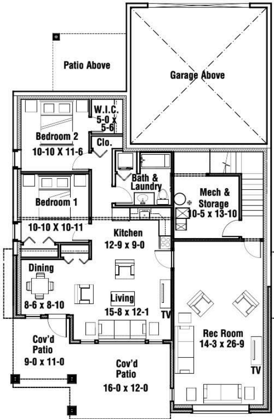
Basement Plan & Secondary Suite 1615 Sq.Ft Total 916 Sq.Ft Suite 699 Sq.Ft Rec Room, Mech. & Storage (Optional Open Basement Plan Available)
