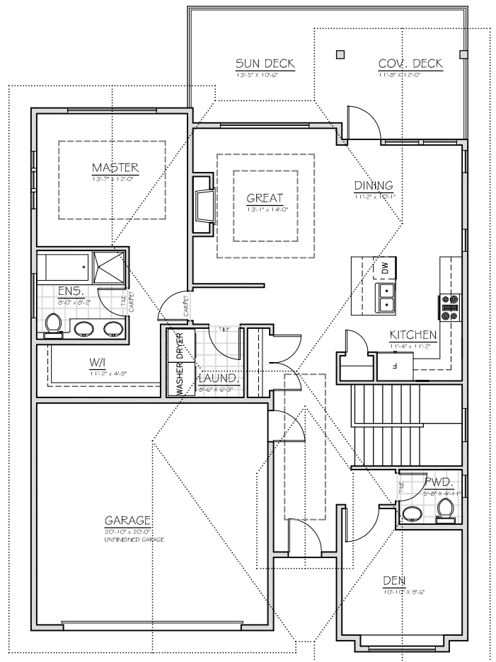
MAIN FLOOR LIVING - 1,329 sq. ft. GARAGE - 447 sq. ft. +/- 9'-0" CEILING
