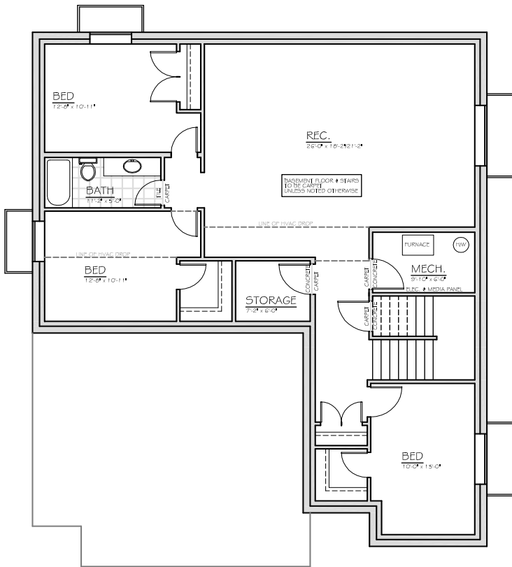
BASEMENT FLOOR LIVING - 1,655 sq. ft.
