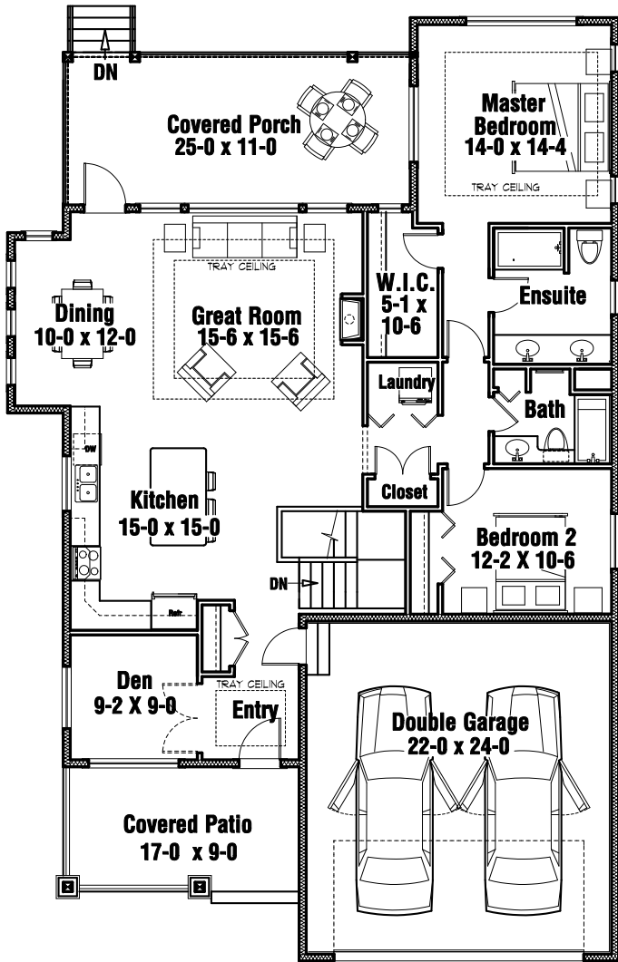
Main Floor Plan - 1622 Sq.Ft.
