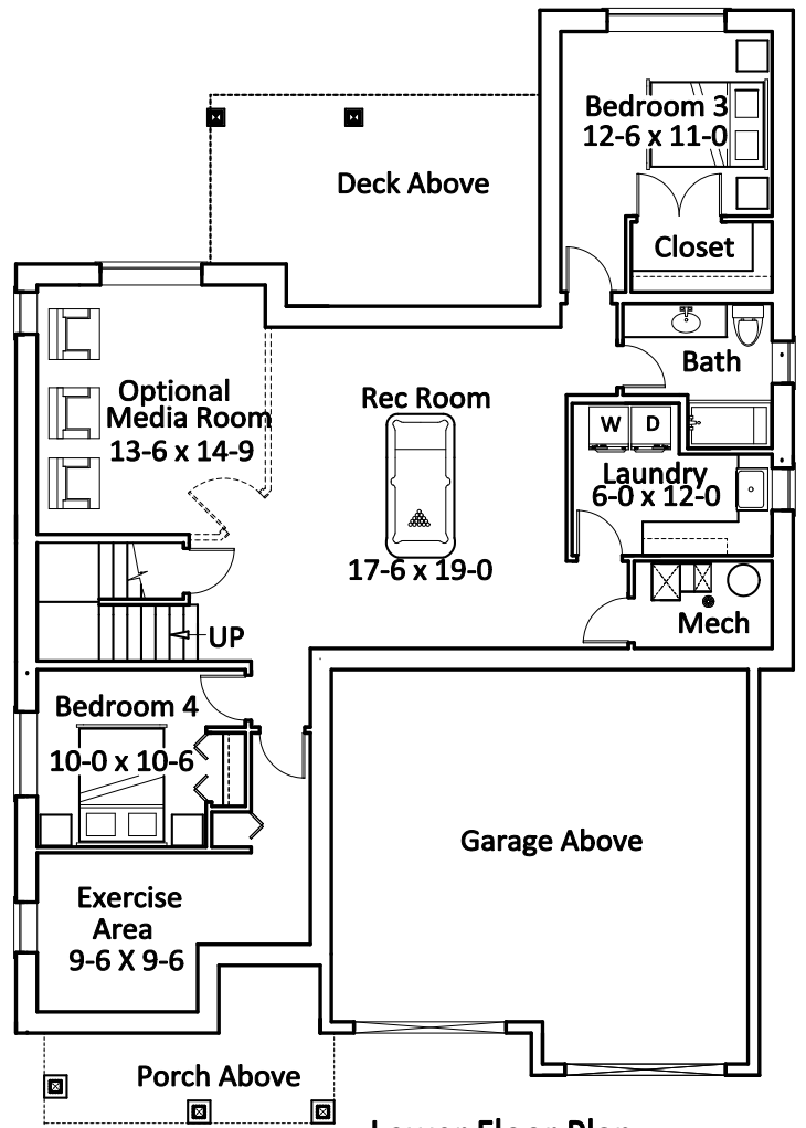
Lower Floor Plan 1590 Sq.Ft Total
