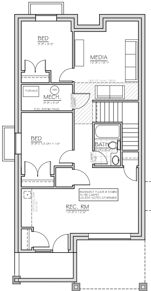
BASEMENT FLOOR
