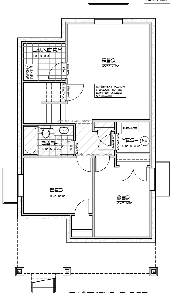
BASEMENT FLOOR LIVING - 925 sq. ft.
