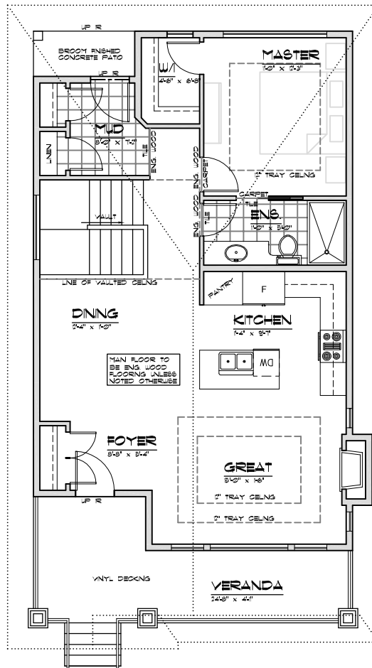
MAIN FLOOR LIVING - 925 sq. ft.
