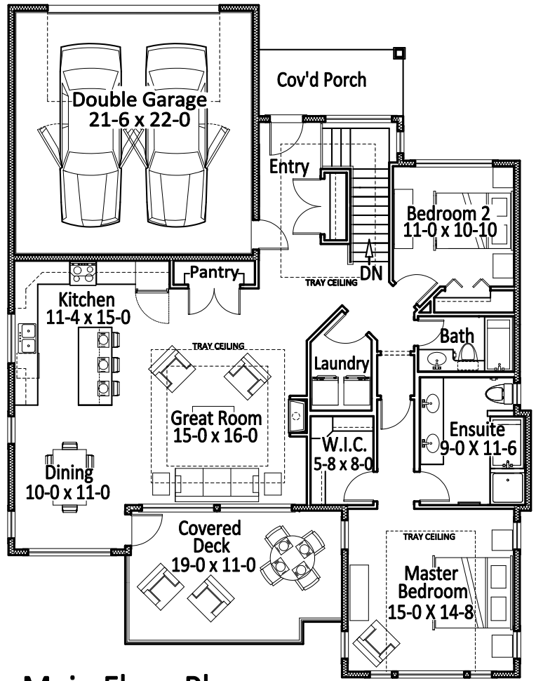
Main Floor Plan 1582 Sq.Ft
