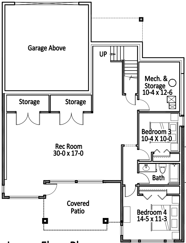
Lower Floor Plan 1582 Sq.Ft
